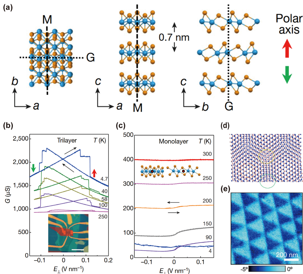
Fig. 10 (a) Top view, side view and front view of the 1T' -WTe 2 homotrimer layer, M represents the mirror plane; G is the sliding plane; red arrow up and green arrow down are polar c -axes. W atoms are in blue; Te atoms are in orange. (b) Conductance G of the undoped trilayer device as E_{\perp} is swept up and down (black arrows). The plots show bi-stability associated with electric polarization up (red arrow) or down (green arrow), at temperatures from 4 K to 300 K (as labelled). Inset is the optical image of a representative double-gated device. (c) Similar measurements on a monolayer 1T' -WTe 2 device (M1), showing no bistability. 173 Reprinted with permission from ref. 173. Copyright 2018, Macmillan Publishers Ltd, part of Springer Nature. (d) Schematic diagram of twisted bilayer h-BN forming moiré superlattice ferroelectricity. 25 Reprinted with permission from ref. 25. Copyright 2017, American Chemical Society. (e) Twisted h-BN ferroelectric domain image with a triangular period. 175 Reprinted with permission from ref. 175. Copyright 2021, The Authors, published by Springer Nature.
