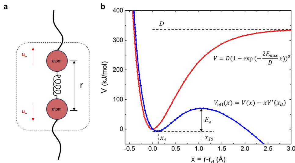
Fig. 6 (a) Schematic illustration for a covalent bond within a polymer chain; (b) undisturbed Morse potential V and effective potential V_{\text{eff}} when mechanical force F is applied to the covalent bond.
