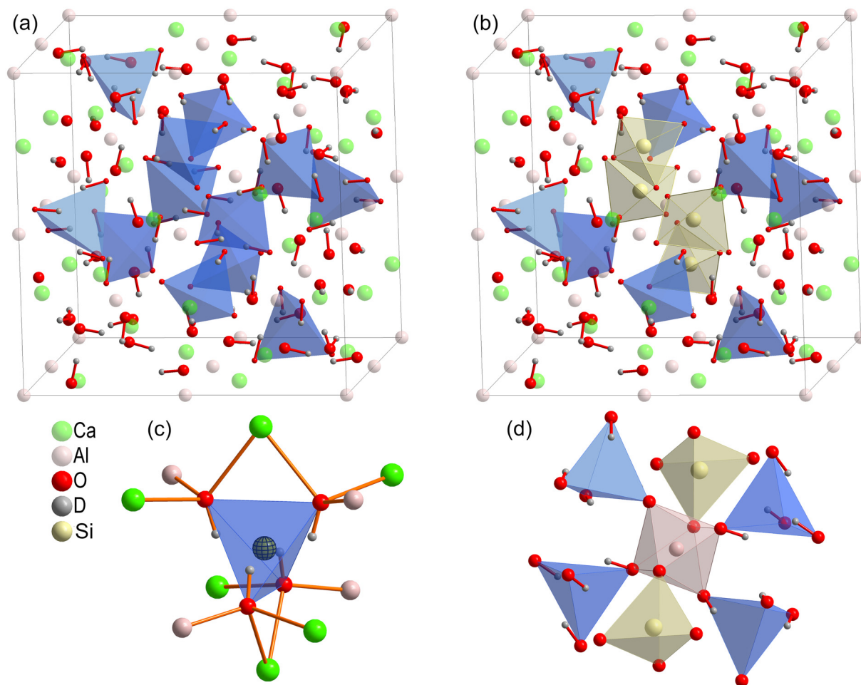
Fig. 1 Comparison of the crystal structures of katoite (a) and partially Si-substituted hydroglossular (b), where 1/3 of (OH) 4 groups are replaced by SiO 4 . The positions of the four hydroxyl groups are highlighted by blue tetrahedra, and yellow tetrahedra represent the SiO 4 units. A close-up of the local structure of the (OH) 4 unit with a "dummy" atom highlighting the position for silicon incorporation is presented in (c). The local structure of the Al atom is depicted in (d).
