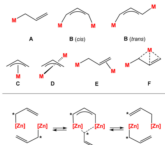
Scheme 13 Top: some of the identified coordination modes of the allyl ligand concerning metal–carbon interactions of \sigma -type ( A : \eta^1 , B : \mu_2-\eta^1:\eta^1 ( cis or trans )), \pi -type ( C : \eta^3 , D : \mu_2-\eta^3:\eta^3 ) or \sigma -type and probably \pi -type ( E : \mu_2-\eta^1:\eta^2 , F : \mu_2-\eta^1:\eta^3 ). Bottom: intermolecular mechanism for allyl exchange in zinc–allyl complexes.
