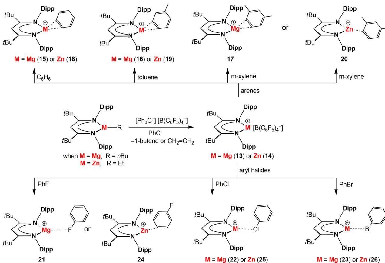
Scheme 6 Synthesis of the “naked” cationic magnesium and zinc complexes 13 and 14 and the [(^t\text{Bu})\text{BDI}^{\text{Dipp}}\text{M}^+(\text{substrate})][\text{B}(\text{C}_6\text{F}_5)_4^-] ( \text{M} = \text{Mg} or \text{Zn} ) complexes 15–26 .
