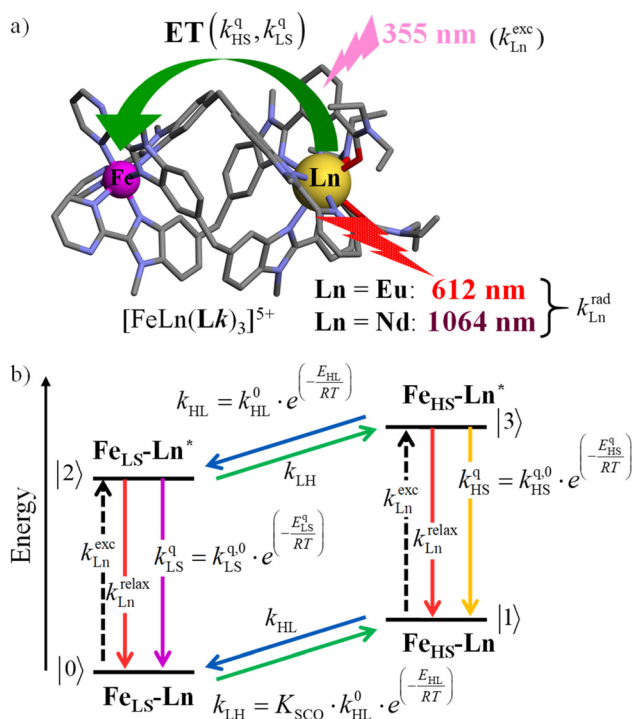
Fig. 8 (a) Fe(II)-modulated light downshifting operating in [\text{Fe}(\text{II})\text{Ln}(\text{Lk})_3]^{5+} helicates (ET = energy transfer) and (b) associated four-states kinetic model.
