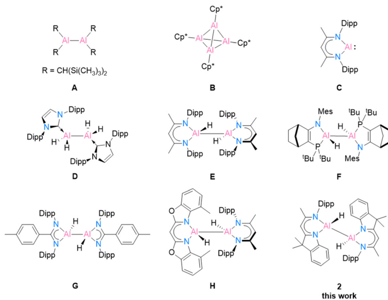
Scheme 1 Selected examples of low oxidation state aluminium compounds A–C, and dialane complexes D–H obtained using [(^{\text{Dipp}}\text{BDIMg})_2] or [(^{\text{Dipp}}\text{BDIAI})] (C) as reducing agents.
