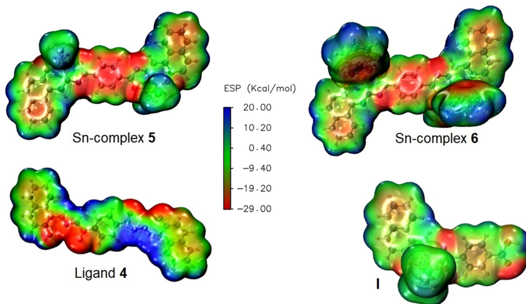
Fig. 13 Electrostatic potential map (EPM) of binuclear Sn-complexes 5 and 6 and their corresponding ligand 4. The EPM of mononuclear Sn complex I ([N-(2-oxido-1-naphthaldehyde)-4-hydroxybenzyhydrazidato]di-nbutyltin) is given for comparison purposes.
