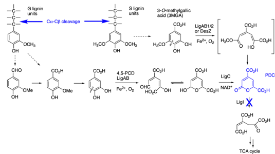
Fig. 9 Generation of pyrone-dicarboxylic acid (PDC) in Novosphingobium aromaticivorans . Gene knockout is shown by a blue cross.
