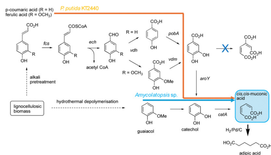
Fig. 11 Production of cis,cis -muonic acid in engineered bacterial strains, showing the routes engineered in P. putida KT2440 (in orange, also for C. glutamicum and N. aromaticivorans ) and Amycolatopsis sp. (in blue).
