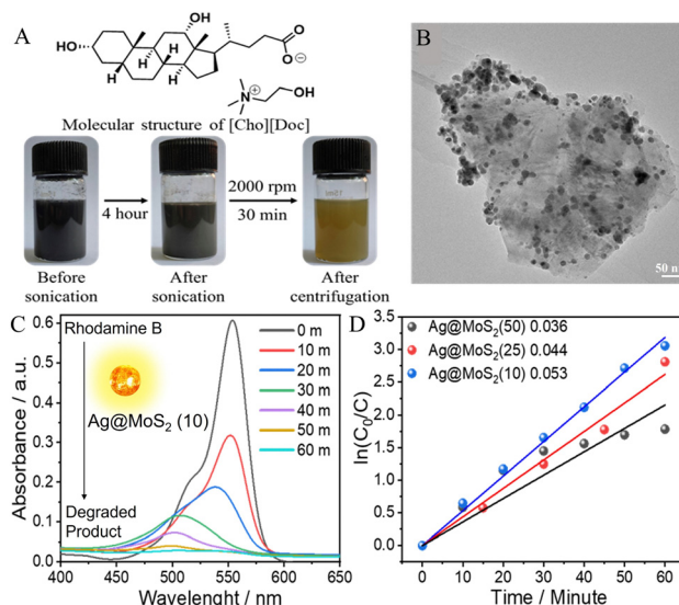
Fig. 14 (A) Molecular structure of [Cho][Doc] and exfoliation of MoS_2 in aqueous [Cho][Doc] ; (B) TEM image showing Ag NPs adhered to the MoS_2 ; (C) time-dependent UV absorbance of RhB in the presence of Ag@MoS_2(10) under sunlight; and (D) comparison of the kinetics of Ag@MoS_2(10) NCs, Ag@MoS_2(25) NCs and Ag@MoS_2(50) NCs. Adopted from ref. 161 with permission. Copyright 2024 Elsevier B.V.
