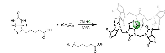
Scheme 1 Synthetic scheme of biotin[6]uril reported by Pittelkow and colleagues. Image reproduced from ref. 116 with permission from The Royal Society of Chemistry.
