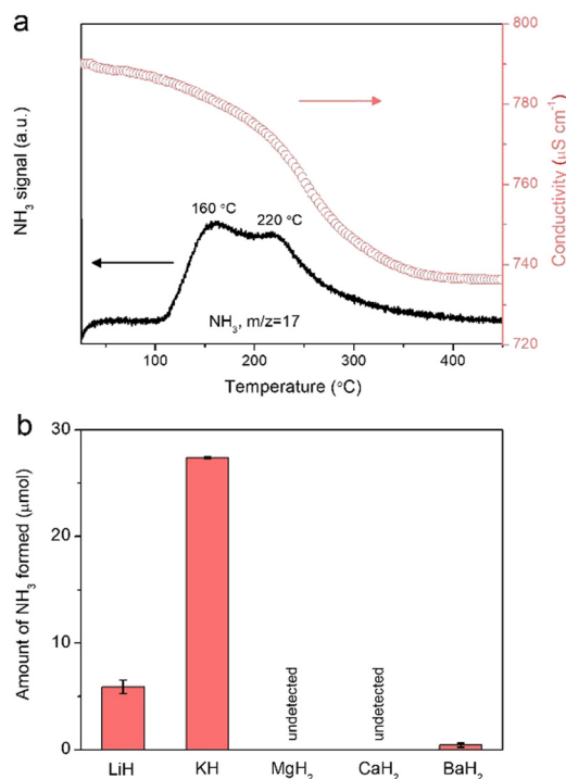
Fig. 2 (a) Temperature-programmed hydrogenation (TPH) profiles of \text{NH}_3 signal ( m/z = 17 ) and conductivity decrease during the hydrogenation of the nitrogen plasma-treated KH sample. Sample mass is 30 mg. P_{\text{H}_2} is 1 bar. \text{H}_2 flow rate is 30 \text{mL min}^{-1} . (b) The amounts of fixed N in metal hydrides determined through TPH measurements. Voltage is 12 kV. Sample mass for LiH is 10 mg, and the others are 30 mg.
