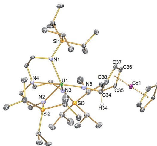
Fig. 1 Molecular structure of 2 with selective labelling at 120 K and displacement ellipsoids at 50%. Hydrogen atoms except for H34 are omitted for clarity.
