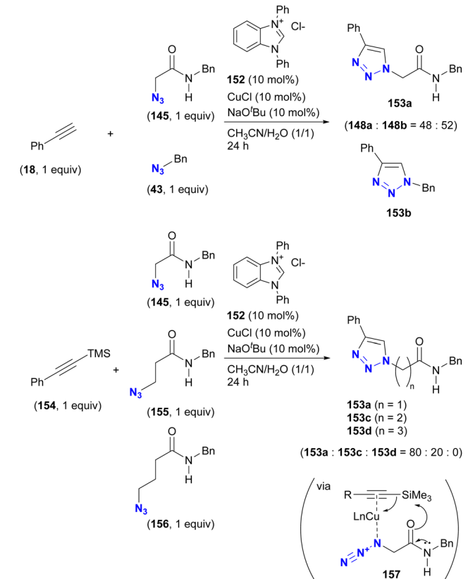
Scheme 29 Copper-NHC-catalyzed CuAAC reactions of silylated and unsilylated alkynes with alkyl azides and the substrate selectivity.
