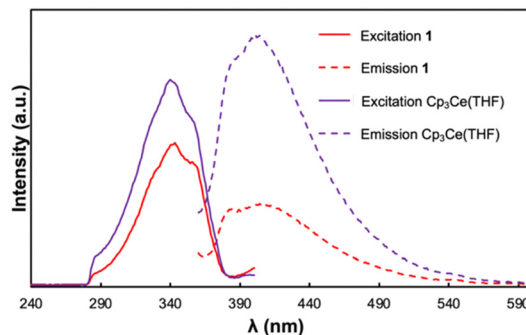
Fig. 3 Photoluminescence spectra of 1 (red) and \text{Cp}_3\text{Ce(THF)} (purple) as a suspension in toluene and a 0.005 mM solution respectively. The excitation spectra at 420 nm emission are shown as solid traces. The emission spectra at 340 nm excitation are shown as dashed traces.
