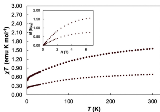
Fig. 2 Variable temperature \chi T measurements of \text{Cp}_3\text{Ce(THF)} (square markers) and 1 (circle markers) at 2 T, variable field magnetization experiments (inset) conducted at T = 2 K.
