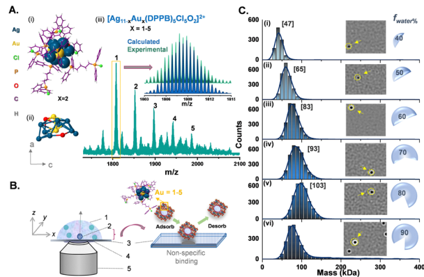
Fig. 1 (A) (i) Calculated structure ( x = 2 ), (ii) the metal, Ag_{11-x}Au_x , core ( x = 2 ), and (iii) ESI MS of [Ag_{11-x}Au_x(DPPB)_5Cl_5O_2]^{2+} ( x = 1–5 ) nanoclusters. In inset, calculated isotopic distribution is stacked with the experimental one. (B) Concept and experimental implementation of MP. Parts in the graphic representation: (1) solvent mixture (sol mix) containing nanoclusters; (2) nanocluster aggregates in solution; (3) glass surface; (4) immersion oil; (5) objective lens. Single-particle landing event on a non-coated cover slide is shown on the right. (C) A stacked plot of the MP histogram of various-sized nanoaggregates with the counts of particle landing events, with varying solvent composition. M_{av} are shown on the spectra as [xx]. The photographs of single-particle binding events on the glass–sol interface during each set of measurements is shown. The corresponding f_{water\%} of solvent mixture is labelled on each histogram.
