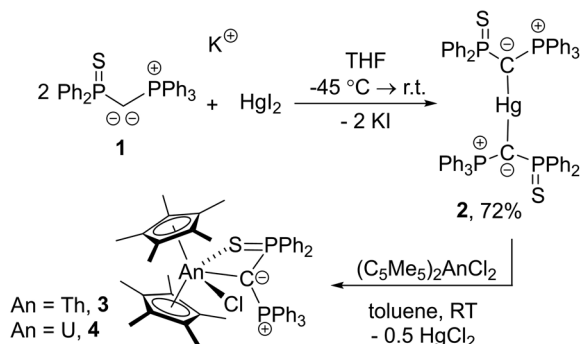
Scheme 1 Synthesis of bis(yliide)mercury, 2 , and Th, 3 , and U, 4 , ylide complexes.
