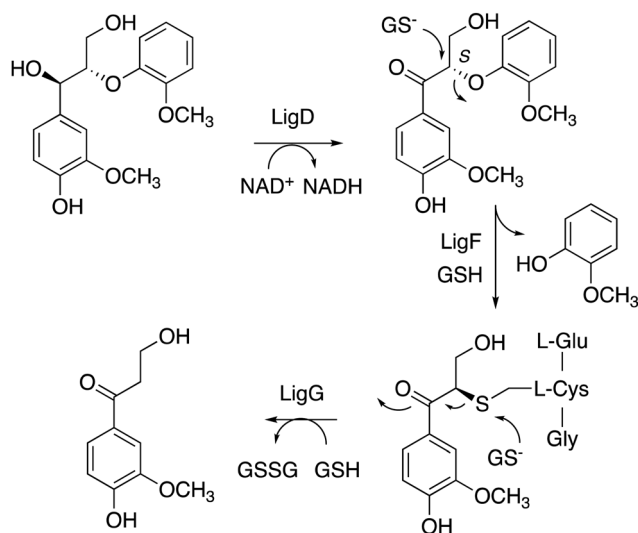
Fig. 5 Mechanism of LigFG \beta -aryl ether cleavage. \text{GS}^- , reduced glutathione; \text{GSSG} , oxidised glutathione. \beta -Esterase LigE catalyses a similar reaction to LigF, on the R enantiomer.
