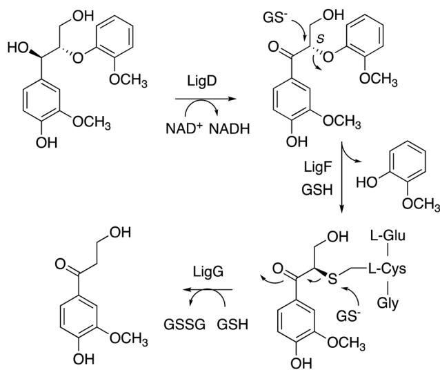
Fig. 5 Mechanism of LigFG \beta -aryl ether cleavage. GS - , reduced glutathione; GSSG, oxidised glutathione. \beta -Esterase LigE catalyses a similar reaction to LigF, on the R enantiomer.
