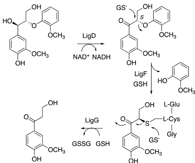
Fig. 5 Mechanism of LigFG \beta -aryl ether cleavage. GS - , reduced glutathione; GSSG, oxidised glutathione. \beta -Esterase LigE catalyses a similar reaction to LigF, on the R enantiomer.
