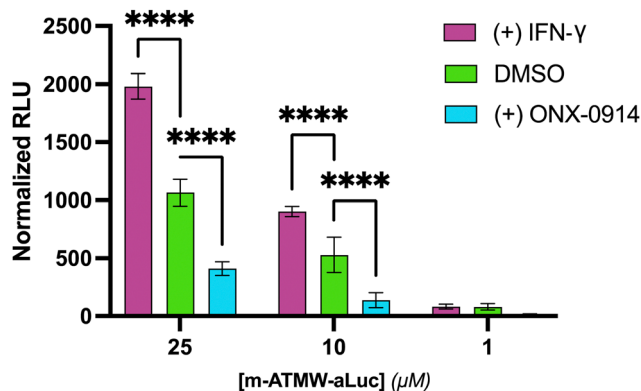
Fig. 3 m -ATMW-aLuc probe incubated with 4T1 cells for 4 h with IFN-gamma (20 ng mL -1 ), DMSO, or ONX-0914 (25 μM) to demonstrate the interaction with the iCP selectively. p < 0.0001 : ****; p < 0.001 : ***; p < 0.01 : **; p < 0.05 : *.
