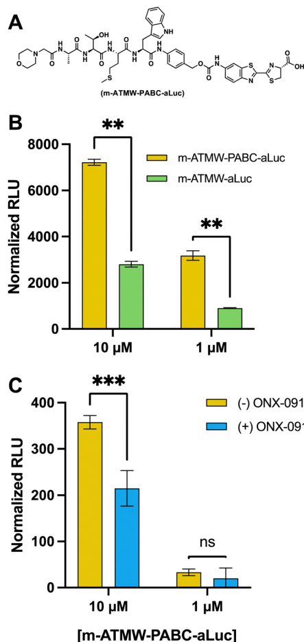
Fig. 5 (A) Structure of m -ATMW-PABC-aLuc. (B) Dose dependent probe analysis with linker (yellow) and without linker (green) with purified iCP. (C) ONX-0914 (25 μM) inhibition of 4T1 cells (blue) compared to DMSO (yellow) prior to addition of probe with linker to demonstrate isoform selectivity.
