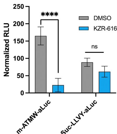
Fig. 4 4T1 cells (20 000 cell per well) incubated with iCP inhibitor KZR-616 (500 nM) followed by incubation with m -ATMW-aLuc (10 μM) or Suc-LLVY-aLuc (10 μM) for 1 h. A one-way ANOVA Dunnett's multiple comparisons test was performed to compare each concentration to DMSO for statistical significance. p < 0.0001 : ****; p < 0.001 : ***; p < 0.01 : **; p < 0.05 : *.
