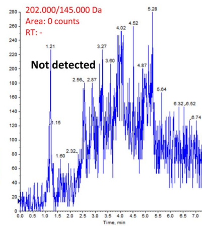
Fig. 2 LC-MS/MS chromatogram of (a) isoproc carb and (b) carbaryl in contaminated robusta coffee during coffee processing.
