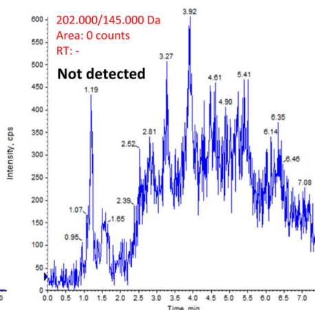
Fig. 2 LC-MS/MS chromatogram of (a) isoproc carb and (b) carbaryl in contaminated robusta coffee during coffee processing.
