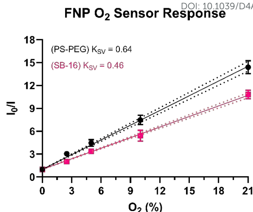
Fig. 4: Stern-Volmer response from the O 2 sensors fabricated using FNP at varying O 2 concentrations. The sensors made with PS-PEG show a more sensitive response to changes in oxygen than its SB-16 counterpart (statistical difference verified via two-tailed t-test, 95% C.I., p = 0.0037 < 0.05 ). Both sensors were excited at 405 nm and the emissions observed 650 nm. Where not visible the error bars are smaller than those of the data points ( n=3 ).
