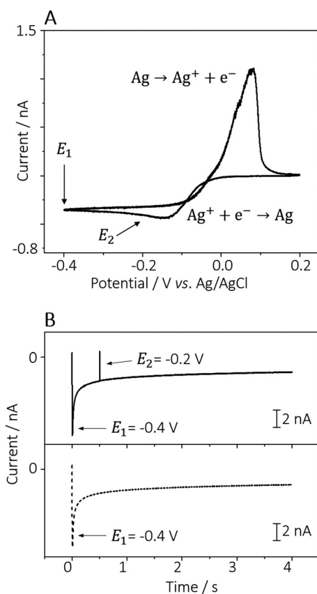
Fig. 1 (A) Cyclic voltammogram of a 0.5 mmol \text{L}^{-1} \text{AgNO}_3 in 50 mmol \text{L}^{-1} \text{KNO}_3 solution recorded at the PDA-modified gold electrode. The potentials applied for the electrodeposition of AgNPs ( E_1 and E_2 ) are highlighted with black arrows. (B) Exemplary current–time curves of the electrodeposition process via a double (continuous line) and single (dotted line) potentiostatic step. Conditions: \text{AgNO}_3 concentration: 0.5 mmol \text{L}^{-1} ; \text{KNO}_3 concentration: 50 mmol \text{L}^{-1} ; SECCM pipette diameter: 5 \mu\text{m} ; working electrode: PDA-modified gold electrode.
