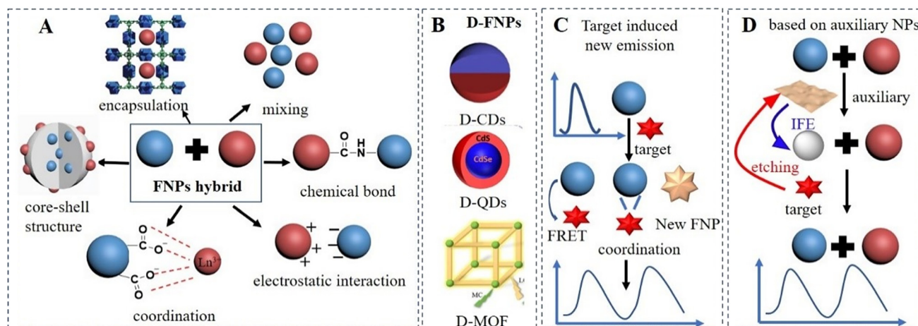
Fig. 2 Design strategies for DRFP. (A) Hybrid nanoparticles. (B) Single nanoparticles with intrinsic dual emission. (C) Single FNP for target-induced new emission and (D) DRFPs based on non-fluorescence auxiliary nanomaterials.
