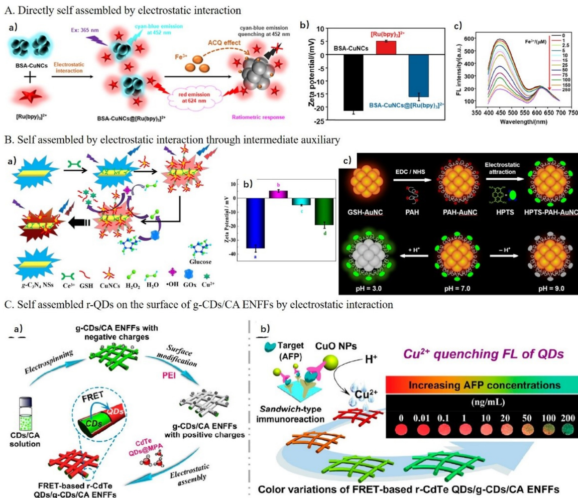
Fig. 7 (A) Construction of DRFP by directly assembling BSA-Cu NCs and [\text{Ru}(\text{bpy})_3]^{2+} by electrostatic interaction for \text{Fe}^{3+} detection. Reproduced with permission from ref. 92. Copyright 2022, Elsevier. (B) The construction of DRFP by the assembly of \text{g-C}_3\text{N}_4 NSs and Cu NCs by electrostatic interaction through an intermediate \text{Ce}^{3+} auxiliary for the detection of \text{H}_2\text{O}_2 . Reproduced with permission from ref. 94. Copyright 2022, Elsevier. (C) The construction of DRFP via the assembly of QDs on the surface of g-CD/CA ENFFs by electrostatic interaction and application of \text{Cu}^{2+} -mediated immunoassay for biomarkers. Reproduced with permission from ref. 97. Copyright 2018, the American Chemical Society.
