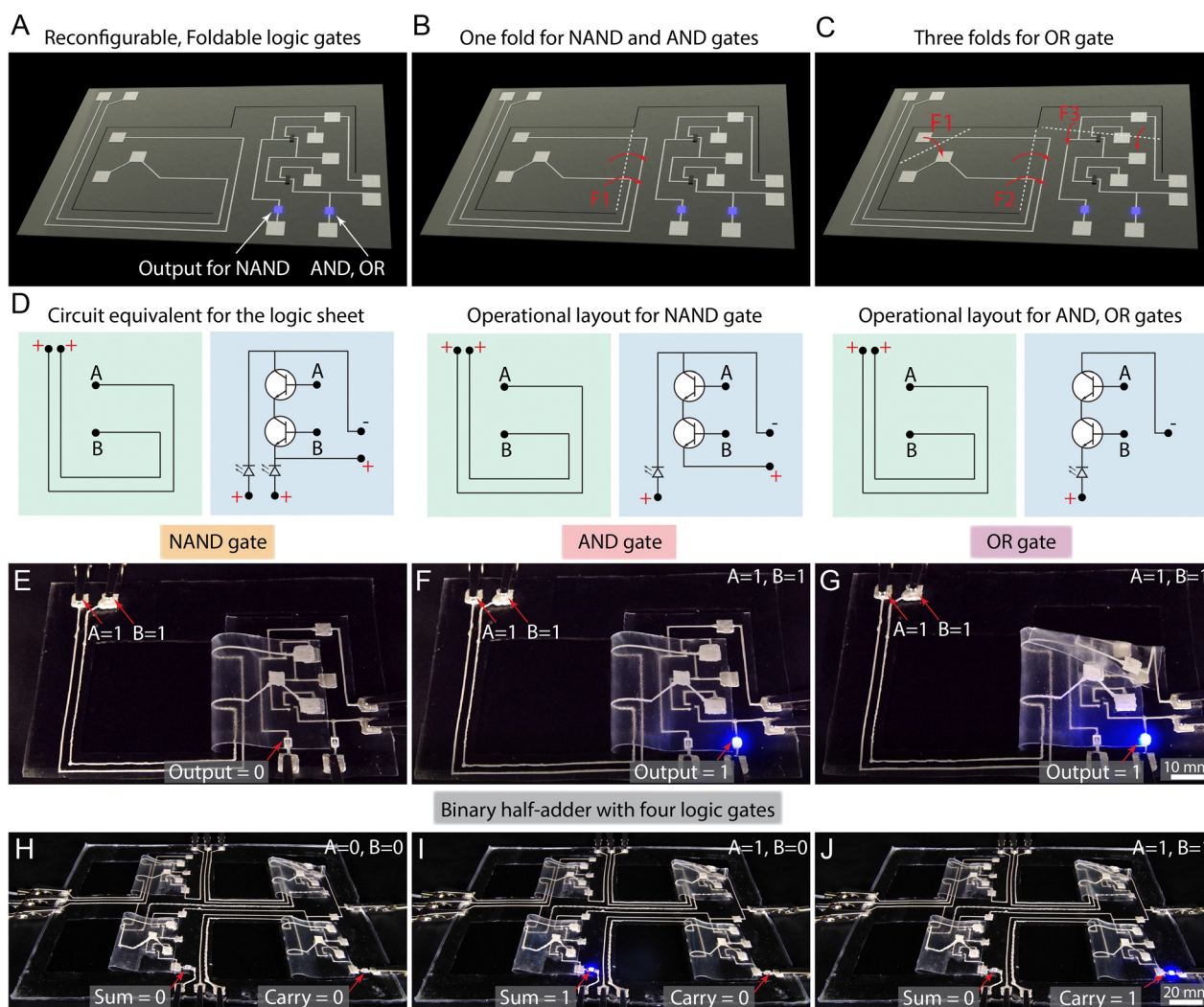
Fig. 4 Reconfigurable, foldable logic through kuttukigami. (A) Schematic of the reconfigurable logic gate circuit with LEDs to indicate binary output of the folding logic with fold lines and folding directional arrows for (B) NAND and AND logic gates. (C) OR logic gate. (D) Circuit equivalent for the logic sheet and operational layouts for individual gates, green represents the input and blue the transistor side. (E)–(G) Images of the fabricated circuit and folds showing the outputs for inputs A = 1 , B = 1 for the respective gates. (H)–(J) Implementation of binary half-adder circuit using four individual reconfigurable circuits the LEDs at the bottom left and the bottom right circuits indicate the sum and carry outputs for the half-adder for different input A , B combinations.
