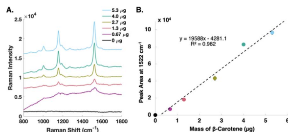
Fig. 3 Raman spectroscopy-based calibration curve for β-carotene on TLC plate. (A) Average Raman spectra from different quantities of β-carotene spotted onto TLC plate using 2 μL drops. Spectra are offset for clarity. (B) Plot of average peak area at 1522 cm -1 as a function of β-carotene mass loaded onto TLC plate. Standard deviations are included as error bars.
