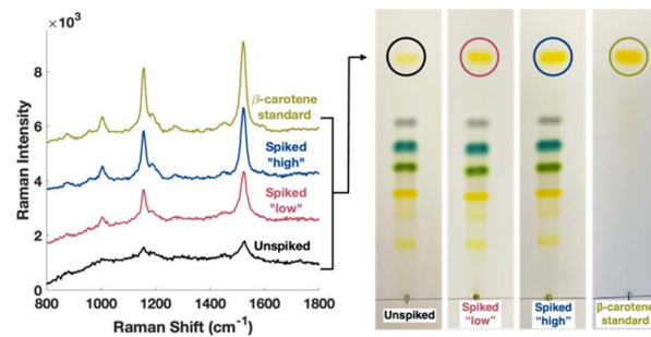
Fig. 2 Average Raman spectra and images obtained from TLC plates spotted with samples of tomato leaf extract, β-carotene-spiked tomato leaf extract, and β-carotene standard (2.7 μg). Spectra are offset for clarity. Drops of 2 μL were used to spot all samples. R f values for all plates are 0.9.
