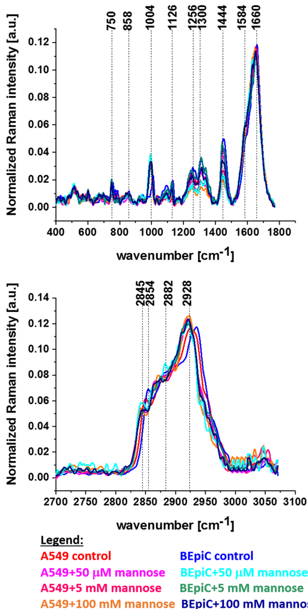
Fig. 6 The average normalized Raman spectra for control A549 cell line (red line); A549 cell line supplemented with 50 μM mannose (magenta line); A549 cell line supplemented with 5 mM mannose (pink line); A549 cell line supplemented with 100 mM mannose (orange line); control BEpiC cell line (blue line); BEpiC cell line supplemented with 50 μM mannose (turquoise line); BEpiC cell line supplemented with 5 mM mannose (dark cyan line); BEpiC cell line supplemented with 100 mM mannose (nary line) in the fingerprint and high-frequency region.
