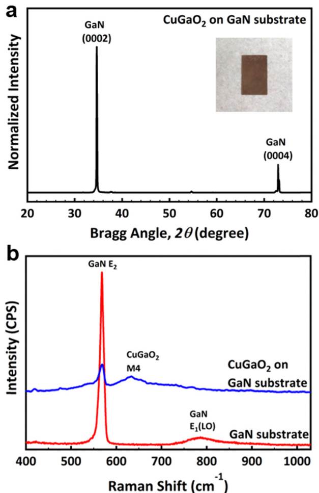
Fig. 2 (a) XRD profile of a \text{CuGaO}_2 film grown on the GaN substrate with a digital photograph of it in the inset, and (b) Raman spectra of the GaN substrate before and after epitaxial growth.
