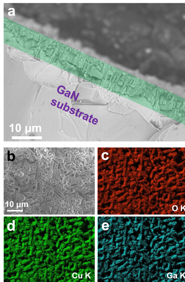
Fig. 3 (a) SEM cross-section image of the film on the substrate, (b) SEM micrograph of the film surface, and EDS mapping of the corresponding elements (c) O K\alpha , (d) Cu K\alpha , and (e) Ga K\alpha .
