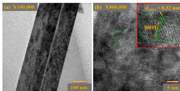
Fig. 4 (a) TEM images of a single \text{TiO}_2 NR, and (b) the corresponding HRTEM image of a single \text{TiO}_2 NR. The inset image of (b) displays the lattice spacing between (101) planes of rutile phase \text{TiO}_2 .
