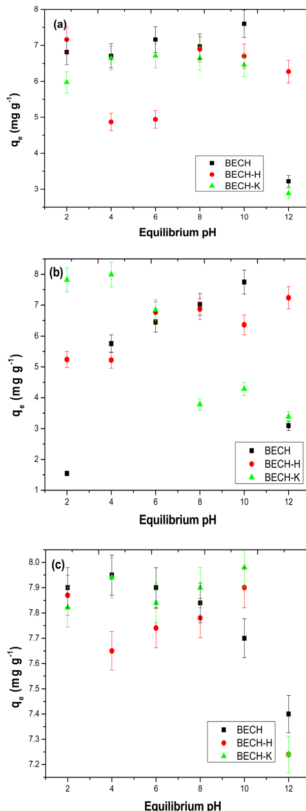
Fig. 8 Effect of pH on the adsorption of (a) ciprofloxacin, (b) tetracycline and (c) bisphenol A (adsorbent mass – 50 mg; pollutant concentration – 40 \text{ mg L}^{-1} ; contact time – 120 min).
