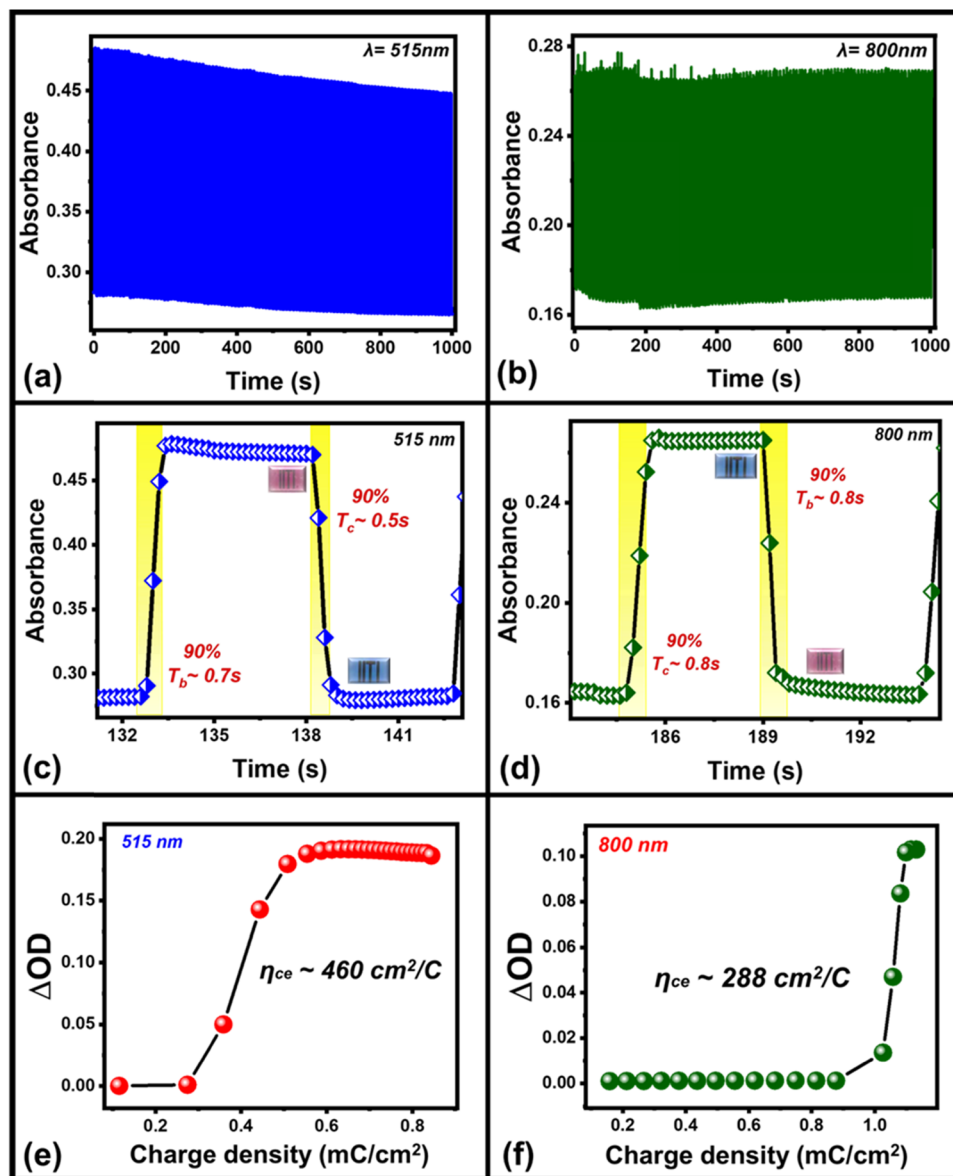
Fig. 4 (a) In situ bias-dependent multiple switching cycles of the device between ON and OFF states in the voltage window ( \pm 1.5 \text{ V} ) in the visible and infrared (IR) wavelength region in (b) and (c) single switching cycle at 515 nm wavelength, (d) response time of the device in the same fixed voltage window at 800 nm wavelength, and the corresponding estimated coloration efficiencies of the device in (e) and (f).
