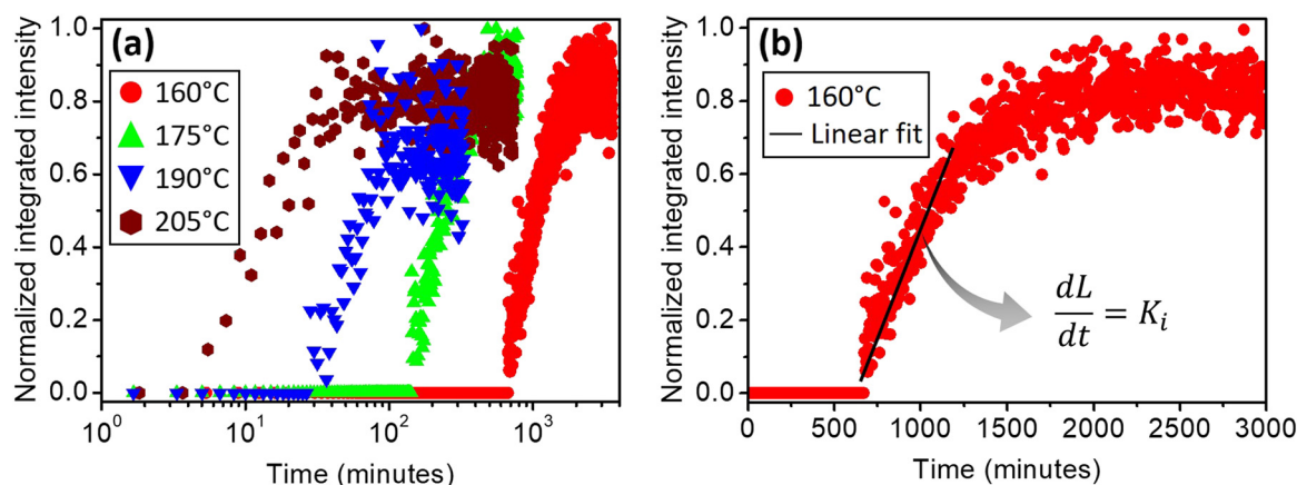
Fig. 3 Normalized integrated intensity f(t) of the \alpha -GeTe(202) diffraction peak versus time recorded during in situ XRD isothermal annealing of the Te-onGe bilayer at various temperatures: (a) versus time in log scale for temperatures between 160 °C and 205 °C; (b) versus time in linear scale at 160 °C, the solid line corresponds to a linear fit of the beginning of the growth.
