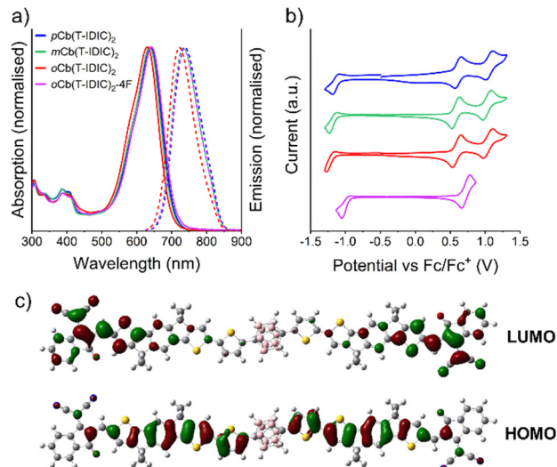
Fig. 1 (a) Absorption and emission spectra of NFA solutions in DCM. (b) Cyclic voltammograms of NFAs, scanning at 0.1 V s −1 and using the Fc/Fc + couple as an internal reference. (c) Frontier molecular orbitals of p Cb(T-IDIC) 2 , as predicted with DFT (B3LYP/6-311G**).
