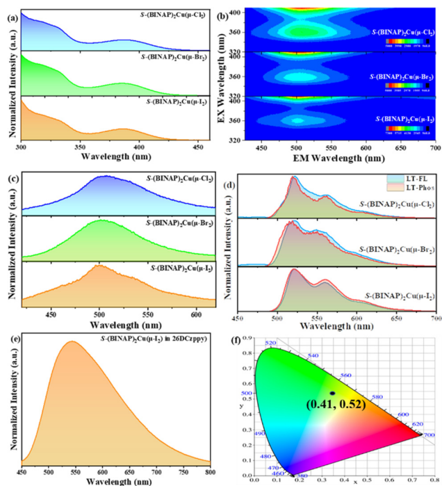
Fig. 2 Photophysical characteristics of S -(BINAP) 2 Cu(μ-Cl 2 ), S -(BINAP) 2 Cu(μ-Br 2 ) and S -(BINAP) 2 Cu(μ-I 2 ) dimers: (a) UV-vis absorption, (b) 3D maps and (c) emission spectra in CH 2 Cl 2 ( 1 \times 10^{-5} mol L -1 ) at room temperature; (d) fluorescence and phosphorescence spectra at 77 K in CH 2 Cl 2 ( 1 \times 10^{-5} mol L -1 ); (e) emission spectrum and (f) CIE coordinates of the S -(BINAP) 2 Cu(μ-I 2 ) doped film in 2,6DCzppy.
