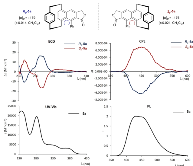
Fig. 1 Chiroptical properties of pCp-based naphthalenes S p - 5a and R p - 5a . UV-Vis, PL, ECD and CPL spectra were recorded in CH 2 Cl 2 (10 -5 M solutions, \lambda_{\text{ex}} = 365 nm).
