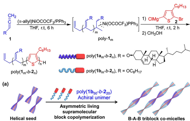
Fig. 13 Synthesis of P3HT block copolymers (top). Schematic illustration of asymmetric living supramolecular polymerization of achiral poly(1b 50 -b-2 20 ) unimer initiated by right-handed helical seed micelle of poly(1a 80 -b-2 20 ) (down). Copyright 2022, WILEY-VCH.
