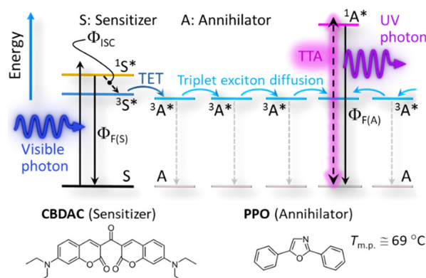
Scheme 1 Schematic energy diagram of TTA-UC in this study. X, 1 X*, and 3 X* (X = S or A: sensitizer or annihilator) denote the ground state, excited singlet state, and excited triplet state, respectively. TET: triplet energy transfer; TTA: triplet–triplet annihilation. Bottom shows the sensitizer and annihilator selected in this study.
