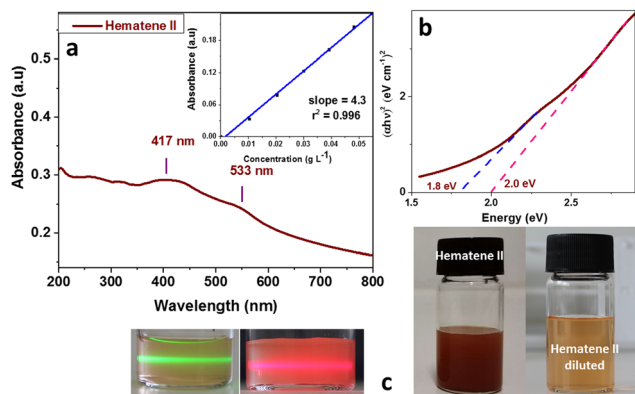
Fig. 1 Hematene II: (a) UV-Vis spectrum in water dispersion. (b) Tauc plot diagram for direct transitions. (c) Photos of Hematene II in water as a subject of the Tyndall effect with green and red laser beams and concentrated and diluted water solutions. Inset, the calibration curve of Hematene II.
