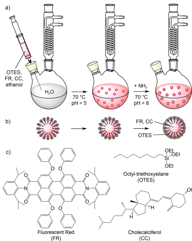
Fig. 1 Schematic illustration of the water-based injection-based synthesis of FR/CC@SiO 2 core-shell nanoparticles: (a) synthesis, (b) structure of nanoparticle, (c) structure of used molecules.
