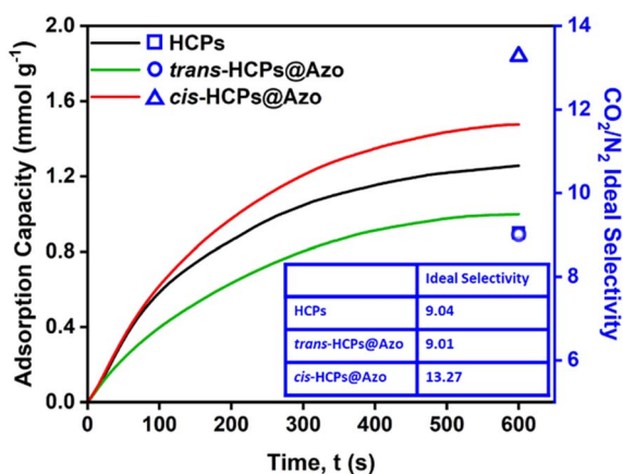
Fig. 3 CO 2 adsorption profiles of (black) HCPs, (green) visible light irradiated trans -HCPs@Azo and (red) UV light irradiated cis -HCPs@Azo using a flow rate of 10 mL min -1 , pure CO 2 gas, at room temperature and atmosphere pressure. CO 2 /N 2 ideal selectivities of HCPs, trans -HCPs@Azo and cis -HCPs@Azo were obtained using CO 2 and N 2 pure gas adsorption capacities after 600 s (Table S2†). 43,44
