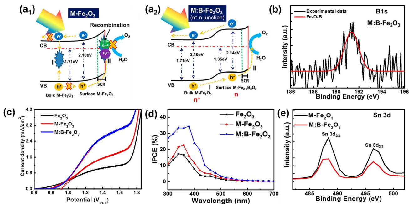
Fig. 10 (a) Schematic illustration of an energy band diagram and charge transfer process of (a 1 ) M\text{-Fe}_2\text{O}_3 and (a 2 ) M\text{:B-Fe}_2\text{O}_3 , (b) XPS B 1s spectra, (c) J - V curves, (d) IPCE, and (e) XPS Sn 3d spectra. Reproduced from ref. 44 with permission from American Chemical Society, Copyright 2018.
