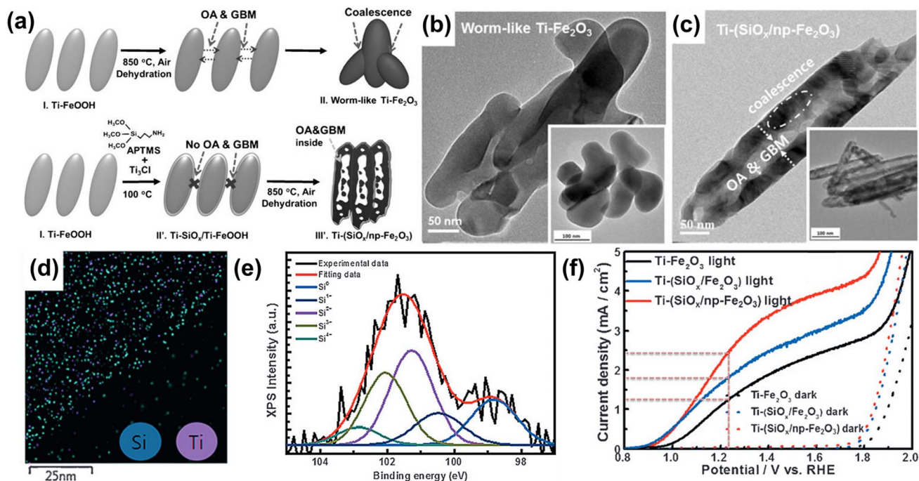
Fig. 5 (a) The fabrication procedures for conventional worm-like \text{Ti-Fe}_2\text{O}_3 and \text{Ti-(SiO}_x\text{)}_n layer-coated porous hematite ( \text{Ti-(SiO}_x\text{)/Fe}_2\text{O}_3 ). TEM image of (b) a worm-like \text{Ti-Fe}_2\text{O}_3 and (c) \text{Ti-(SiO}_x\text{)/np-Fe}_2\text{O}_3 . (d) EDS mapping images of Si and Ti of \text{Ti-(SiO}_x\text{)/np-Fe}_2\text{O}_3 . (e) XPS Si 2p spectra of \text{Ti-(SiO}_x\text{)/np-Fe}_2\text{O}_3 . (f) J - V curves of \text{Ti-Fe}_2\text{O}_3 , \text{Ti-(SiO}_x\text{)/Fe}_2\text{O}_3 , and \text{Ti-(SiO}_x\text{)/np-Fe}_2\text{O}_3 under 1 sun and dark conditions with a three-electrode system. Reproduced from ref. 52 with permission from Wiley-VCH, Copyright 2016.
