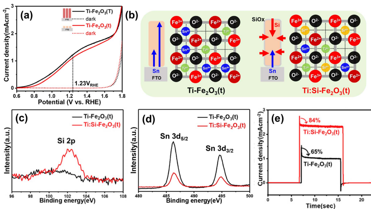
Fig. 11 (a) J - V curves of \text{Ti-Fe}_2\text{O}_3(\text{T}) and \text{Ti-Fe}_2\text{O}_3(\text{t}) under 1 sun and dark conditions. (b) Schematic diagram of decreased metal dopants ( \text{Sn}^{4+} and \text{Ti}^{4+} ) through non-metallic Si doping in \text{Ti:Si-Fe}_2\text{O}_3(\text{t}) . XPS spectra of (c) Si 2p, and (d) Sn 3d. (e) Transient photocurrent density curves (0.001 point per s) measured at 1.23 V_{\text{RHE}} of \text{Ti-Fe}_2\text{O}_3(\text{t}) and \text{Ti:Si-Fe}_2\text{O}_3(\text{t}) . Reproduced from ref. 58 with permission from Elsevier, Copyright 2020.
