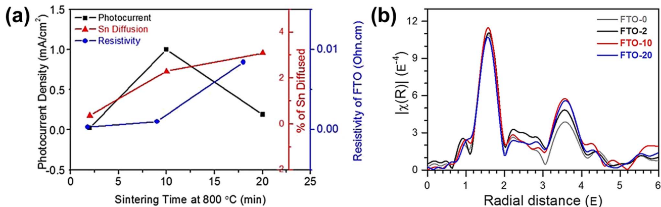
Fig. 8 (a) Photocurrent density ( \text{mA cm}^{-2} ), atomic percent of Sn diffusion of hematite photoanodes, and resistivity of the FTO substrate sintered at 800\text{ }^{\circ}\text{C} for 2, 10, and 20 min. k^3 -weighted Fourier transforms for (b) Sn K-edge EXAFS of FTO substrates sintered at 800\text{ }^{\circ}\text{C} for 0, 2, 10, and 20 min. Reproduced from ref. 62 with permission from American Chemical Society, Copyright 2015.
