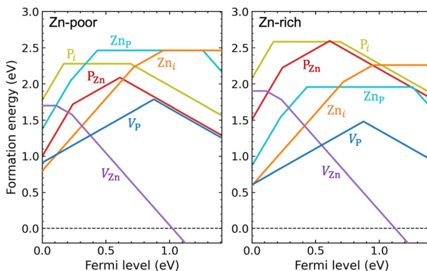
Fig. 1 Formation energies as a function of Fermi level for intrinsic point defects in Zn_3P_2 , under Zn-poor/P-rich (left) and Zn-rich/P-poor (right) conditions. The zero of the Fermi level is set at the VBM and the upper bound corresponds to the conduction-band minimum (CBM). For the same Fermi-level value, only formation energy for the most stable charge state is shown, i.e., V_{Zn} : 0, –, 2–; V_P : +, –, 2+; Zn_i : 2+, +, 0; P_i : 3+, 0, –, 2–; Zn_P : 3+, 2+, 0, 2–; P_{Zn} : 3+, +, –, 2–. Kinks in each curve indicate transitions between different charge states (values of the thermodynamic transition levels are also listed in Table S1 of the ESI † ).
