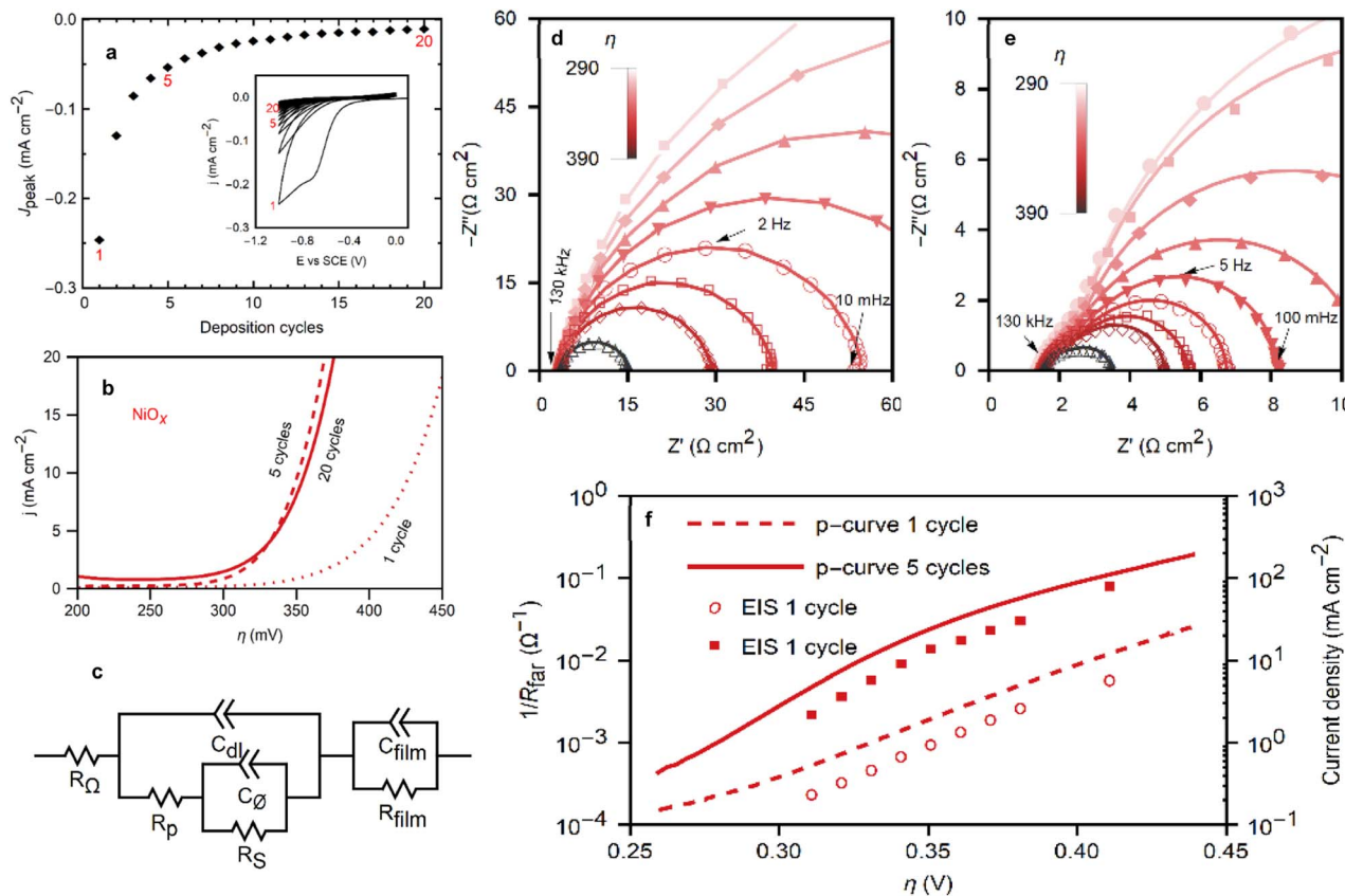
Fig. 5 (a) The peak currents of each deposition cycle from the inset are plotted with cycles 1, 5 and 20 highlighted and (inset) cyclic voltammograms at 20 \text{mV s}^{-1} of the deposition of the nickel oxides over 20 cycles. (b) Polarization curves for the OER with \text{NiO}_x films deposited from 1, 5, and 20 cycles. (c) Equivalent circuit for the impedance process adapted from Lyons et al. 38 EIS Nyquist plots of \text{NiO}_x films ((d) deposited with 1 cycle, (e) deposited with 5 cycles) on GCE in 1 M KOH at applied overpotentials ranging from 290 mV to 390 mV. (f) Tafel plots made from EIS and dc polarization data of \text{NiO}_x of films deposited from 1 and 5 cycles.
