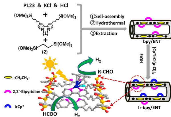
Scheme 14 Synthesis of \text{Ir-bpy/ENT} and photocatalysis with \text{Ir-bpy/ENT} , where ENT is an ethenyl-bridged organosilica nanotube. Reprinted from ref. 118 with permission from Elsevier (Copyright 2018).
