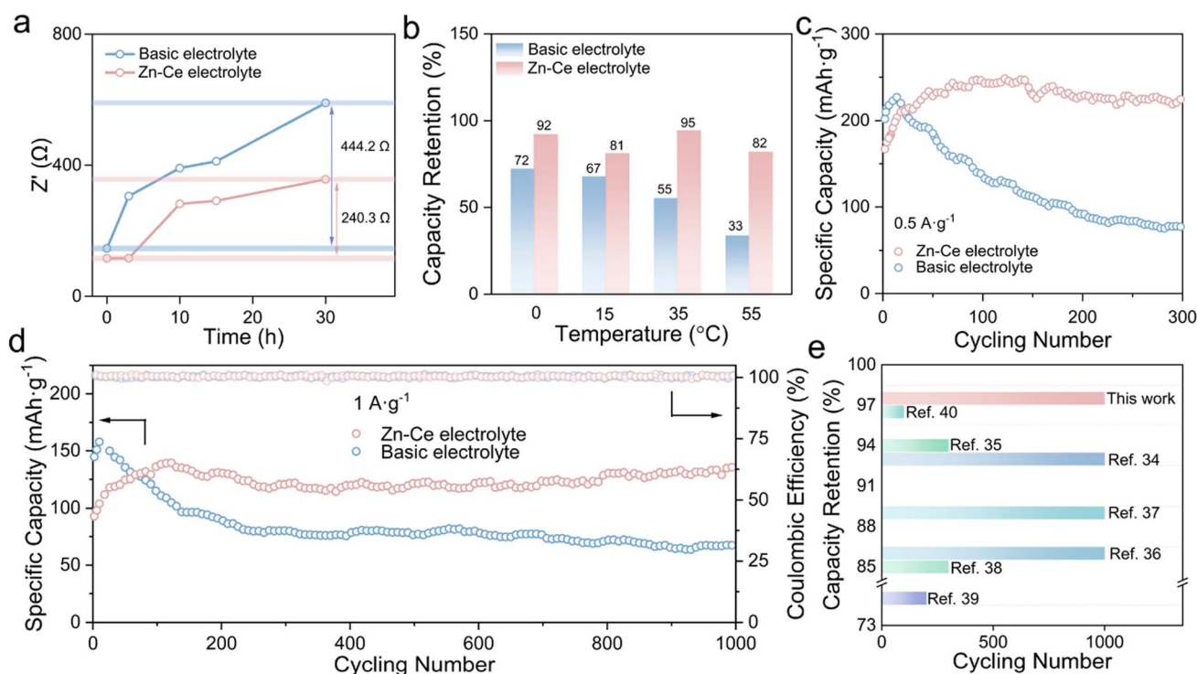
Fig. 4 Comparison of the electrochemical performance of Zn/MnO 2 batteries. (a) Changes in R_{ct} values of Zn/MnO 2 batteries with the basic electrolyte and Zn–Ce electrolyte during 30 h at room temperature. (b) Capacity retention of Zn/MnO 2 batteries with the basic electrolyte and Zn–Ce electrolyte after 200 cycles at 0, 15, 35, and 55 °C. (c and d) Long cycling performance of Zn/MnO 2 batteries with the basic electrolyte and Zn–Ce electrolyte at 0.5 and 1.0 A g -1 . (e) Comparison of electrochemical performance of the Zn/MnO 2 battery based on the Zn–Ce electrolyte with other Zn/MnO 2 batteries reported previously. 34–40
