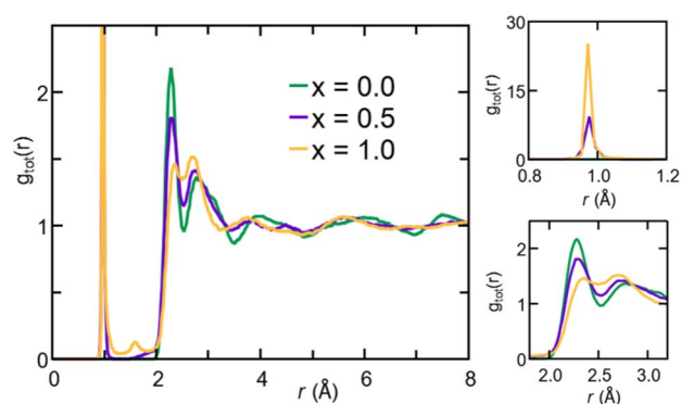
Fig. 3 (Color online) Left: Total pair correlation functions for amorphous \text{Na}_{3-x}\text{OH}_x\text{Cl} ( x = 0 , x = 0.5 , and x = 1 ) obtained at T = 300 \text{ K} . Right: Zoomed-in view of the 0.8\text{--}1.2 (top) and 1.8\text{--}3.2 (bottom) ranges, respectively.
