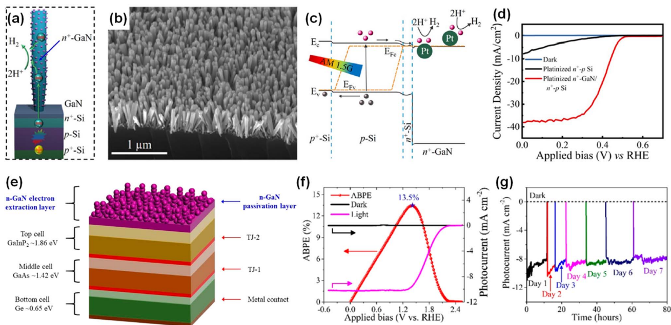
Fig. 10 (a) Schematic of GaN-nanowire-protected n^+ - p Si photocathode with Pt cocatalysts. (b) SEM image of GaN/Si photocathode. (c) Schematic of the energy band diagram of Pt-decorated GaN/Si photocathode under light illumination. (d) LSV curves measured under AM 1.5G 1 sun illumination in 0.5 M \text{H}_2\text{SO}_4 . Reproduced with permission from ref. 97. Copyright (2018) American Chemical Society. (e) Schematic illustration of the \text{GaInP}_2/\text{GaAs}/\text{Ge} triple-junction photocathode protected by GaN nanostructures. (f) Photoelectrochemical \text{H}_2 evolution reaction performance and (g) long-term stability of GaN-protected triple-junction photoelectrode in 0.5 M \text{H}_2\text{SO}_4 under 1 sun illumination. Reproduced with permission from ref. 98. Copyright (2019) American Chemical Society.
