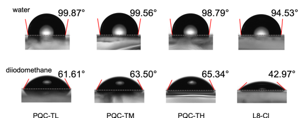
Fig. 4 Contact angle images of various films with water and diiodomethane droplets on top.
