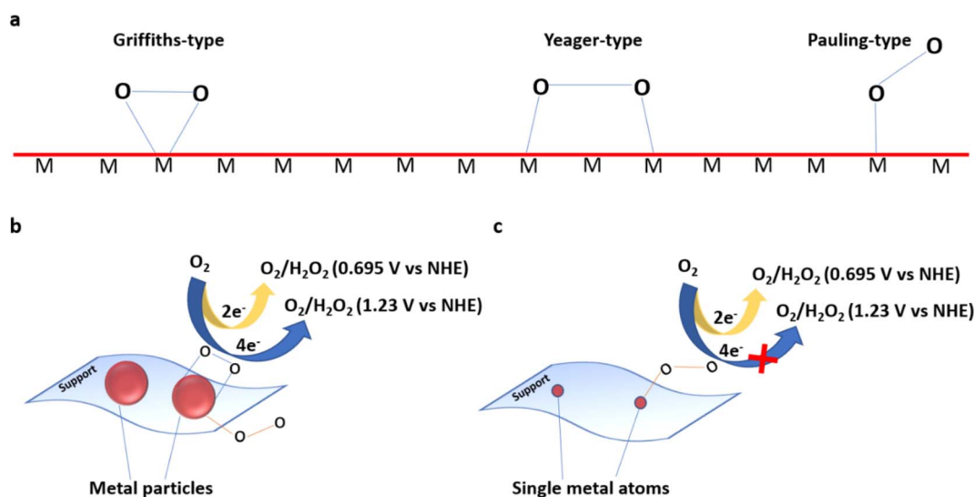
Fig. 23 (a) O 2 adsorption modes on a metal surface, ORR pathways on (b) metal nanoparticles and (c) single metal atom sites.
