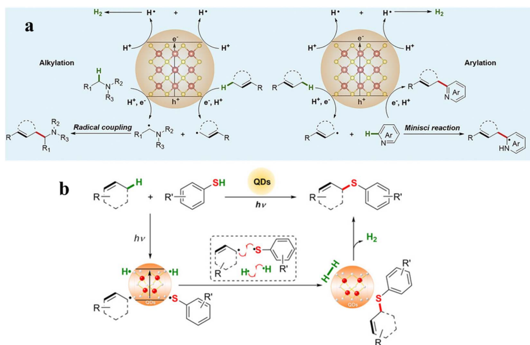
Fig. 10 (a) Alkylation and arylation of an allyl C(sp 3 )–H bond. Reprinted with permission from ref. 122. (b) Direct activation of an allylic C–H bond to form a C–S bond. Reprinted with permission from ref. 123.
